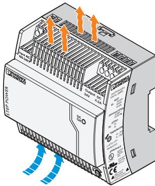
Schematic diagram
